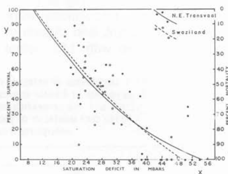
FIGURE 1. Scatter diagrams and regression curves for egg to first instar nymph survival of T. erythrae (Y) against mean saturation deficit (X) for the 3 severest days of count. Northern Transvaal: Y=0.03 X^2 - 4.18 X + 137.77 ; SE of estimate = 19.99 percentage units. Swaziland: Y=0.02 X^2 - 3.70 X + 154.80 ; S.E. of estimate = 17.76 percentage units. After Green and Catling (5).
