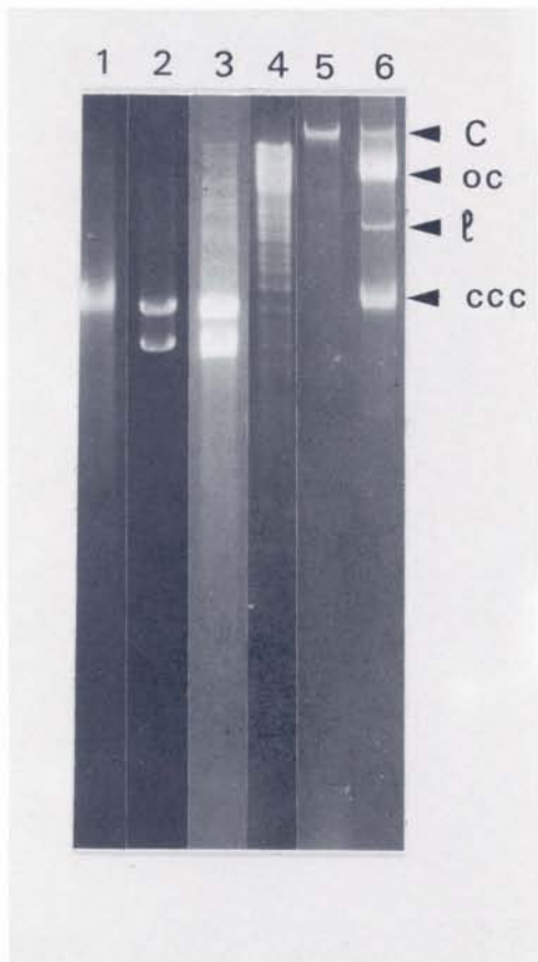
Fig. 1. Electrophoresis of SpV1-78 single stranded, circular DNA (track 1), Eco RI-treated SpV1-78 RF (track 2), Eco RI treated total DNA from SpV1-78-infected S. citri R8A2HP cells (track 3), Eco RI-treated total DNA from uninfected R8A2HP cells (track 4), DNA of cleared lysate from uninfected R8A2HP cells (track 5), DNA of cleared lysate from SpV1-78-infected R8A2HP cells (track 6) on 0.9 % agarose gel.
