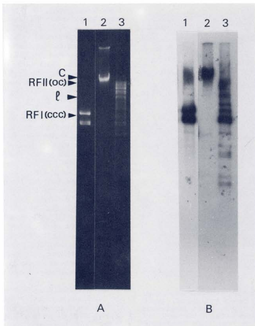
Fig. 2. A) Electrophoresis of EcoRI -treated SpV1-78 RF (track 1), total DNA from S. citri R8A2HP cells (track 2), EcoRI -treated total DNA from R8A2HP cells (track 3) on 1% agarose gel. B) Southern blot hybridization of the DNAs of A with ^{32}\text{P} -labelled SpV1-78 RF as the probe.
