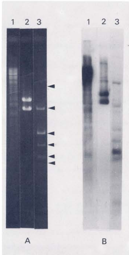
Fig. 3. A) Electrophoresis of Eco RI-treated total DNA of S. citri R8A2HP (track 1), Eco RI-treated SpV1-78 RF (track 2), Taq I-treated SpV1-78RF (track 3) on 1.2% agarose. B) Southern blot hybridization of the DNAs of A with ^{32} P-labelled R8A2HP DNA as the probe. The arrows indicate Taq I restriction fragments.
