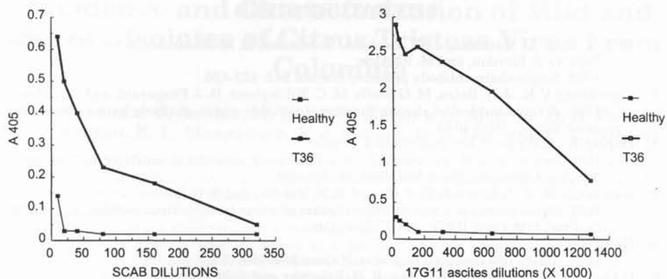
Fig. 5. Comparative titration of SCAB protein from periplasmic extract of E. coli (left panel) in comparison to the parent MAb 17G11 (right panel) by ELISA.
