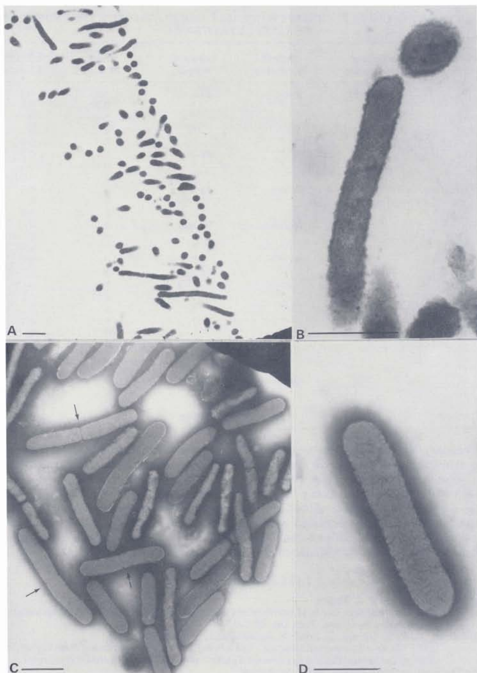
Fig. 3. Electron micrographs of cultured cells of the CVC-bacterium. The bars represent 1 \mu\text{m} (A, C), 0.5 \mu\text{m} (B, D); A, B) cross section through a colony on PW medium; C, D) negative staining, arrows indicate bacteria dividing by binary fission. Note wavy outer wall layer.
